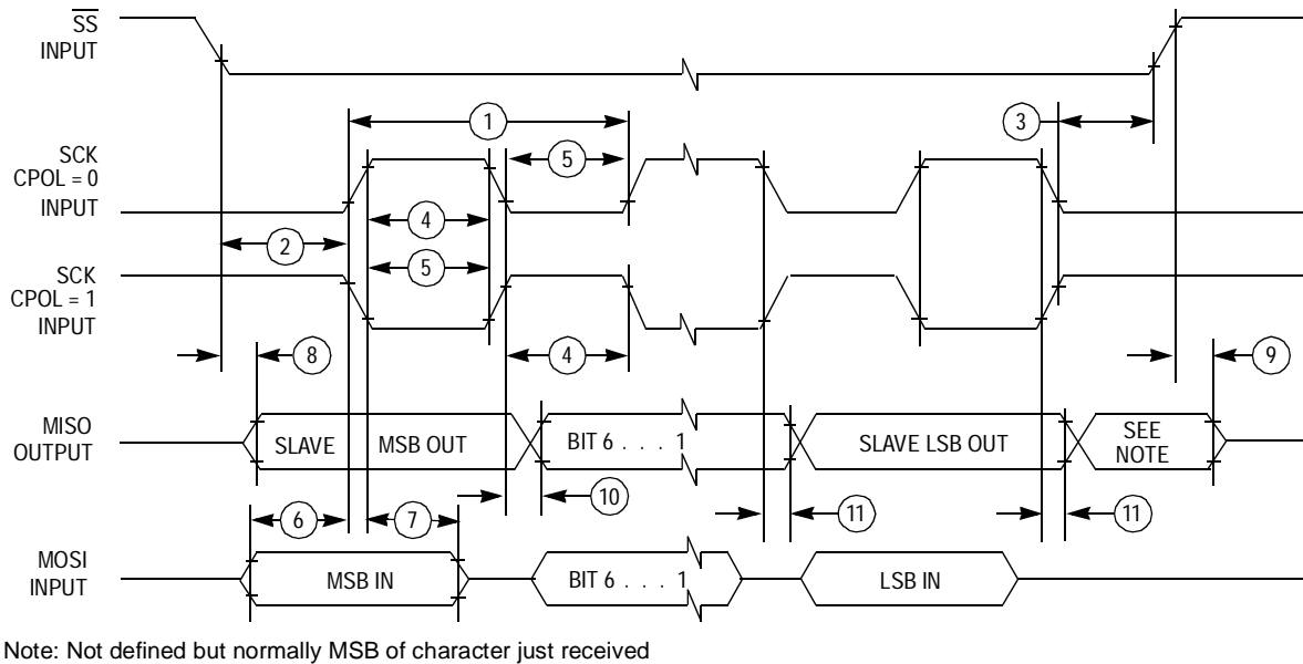
A) SPI Slave Timing (CPHA = 0)
