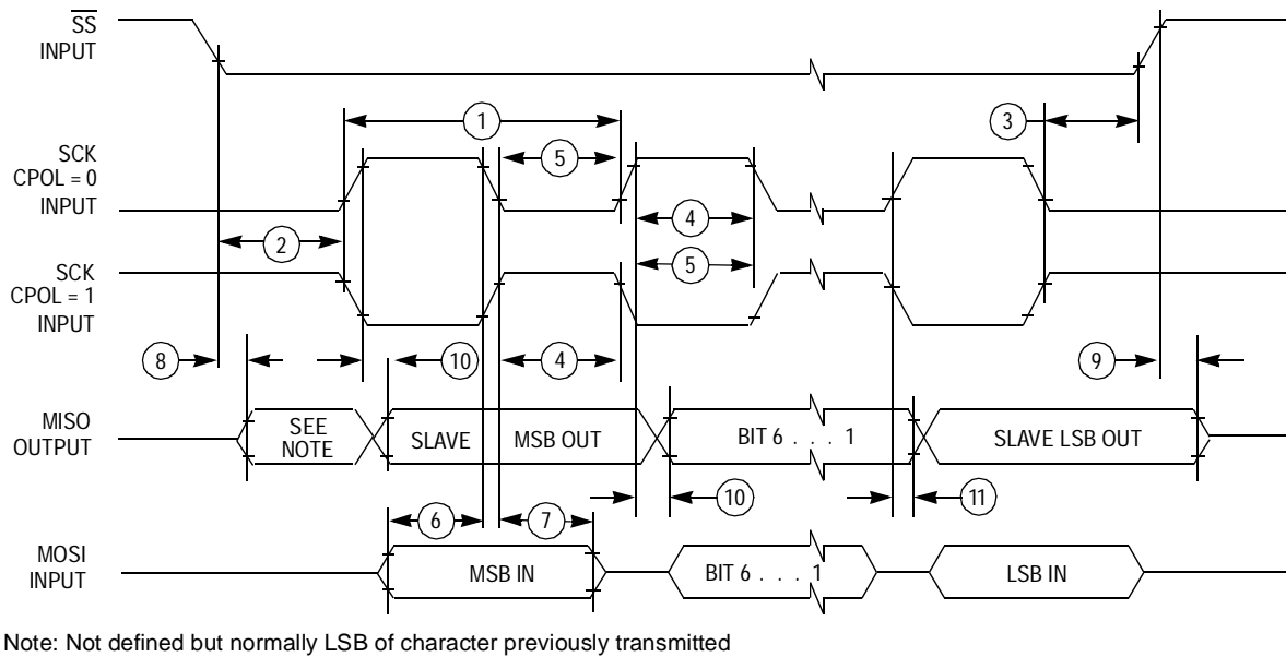
B) SPI Slave Timing (CPHA = 1)
