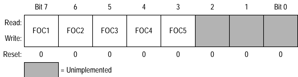
Figure 9-12. Timer Compare Force Register (CFORC)
